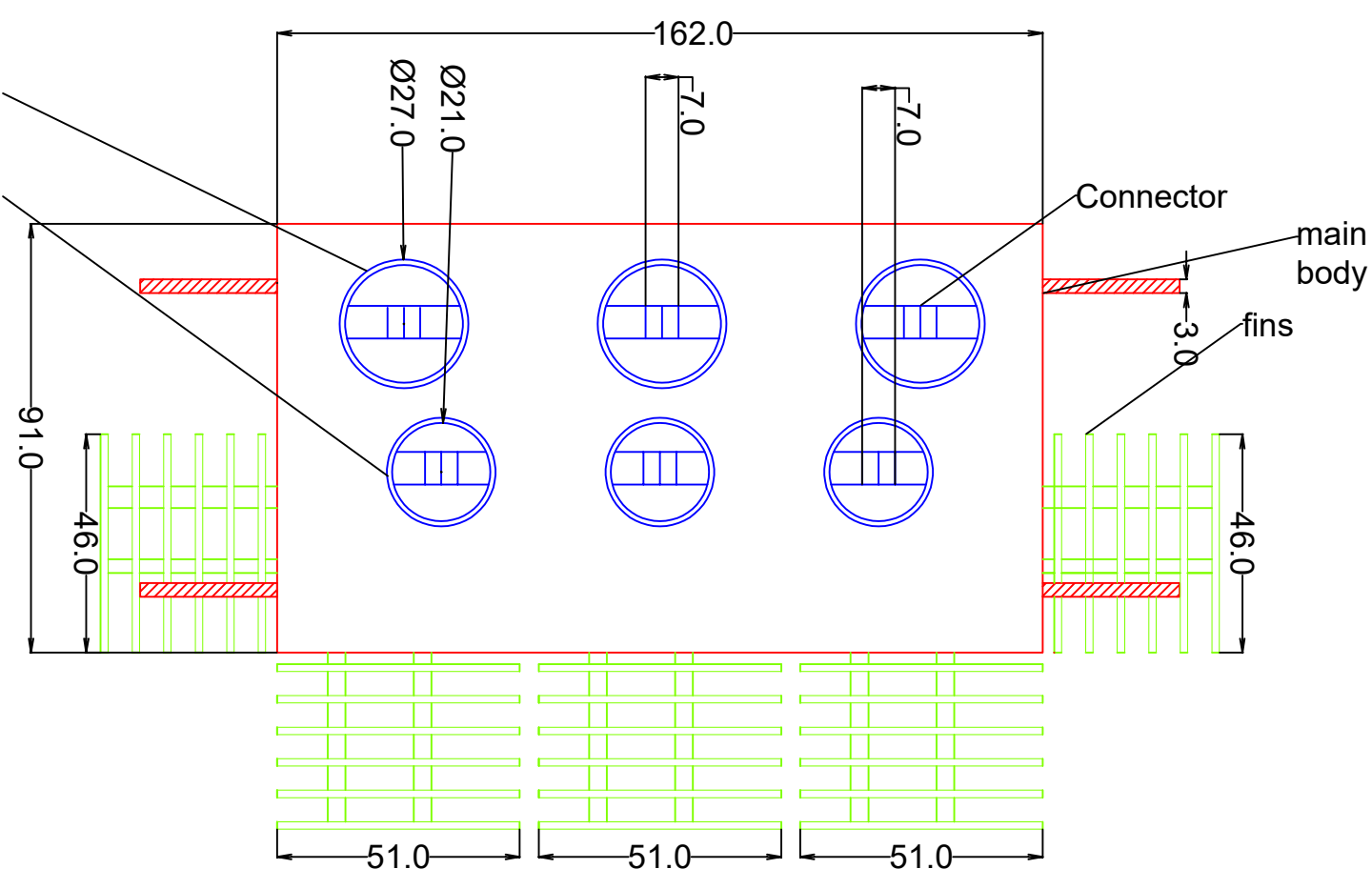
Transformer Top
