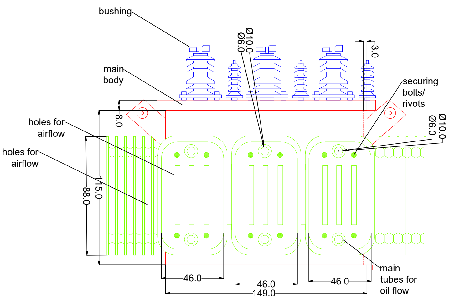
Transformer front
